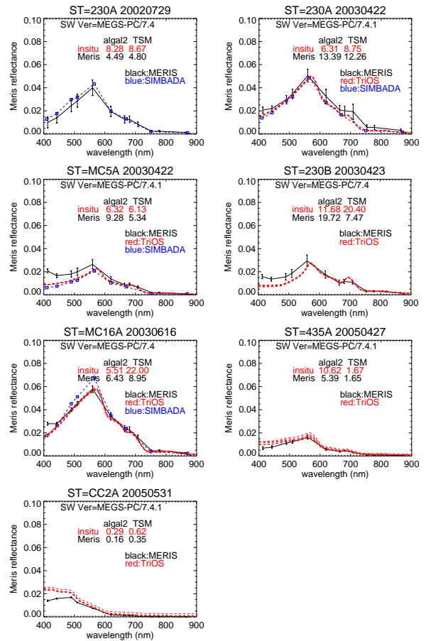
Figure 2. MERIS and seaborne measurements comparison for the seven best match-ups. For the MERIS spectra, mean (solid lines) and standard deviation for the surrounding 3x3 box are indicated. For the TriOS spectra (dotted red lines), the five replicate measurements are shown.
