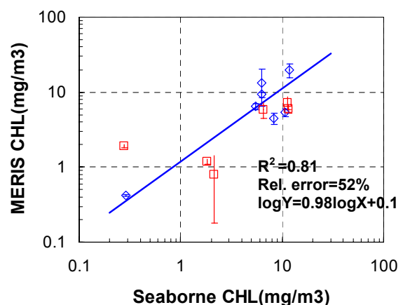
Figure 4. MERIS versus Seaborn Chl: Best match-ups in blue and sun-glint affected match-ups in red. Error bar indicates standard deviation for 3x3 surrounding box.
